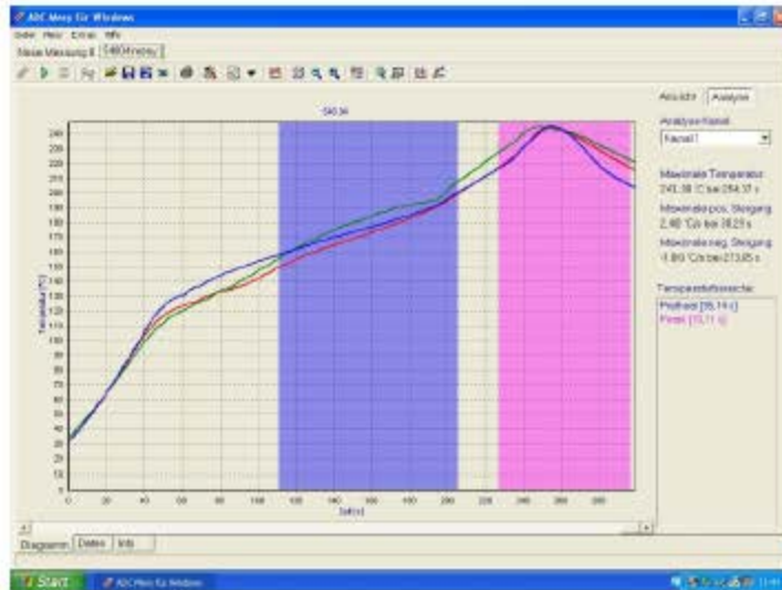
Typical lead free profile 548.04G
