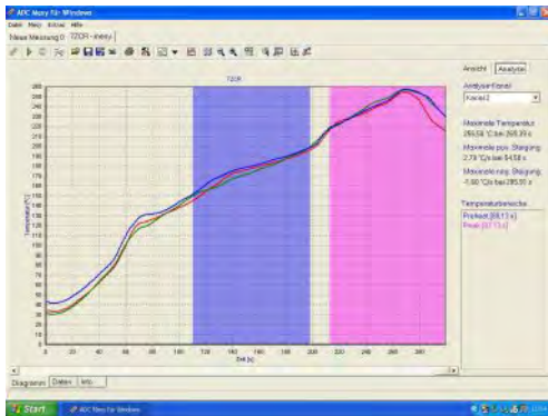
Typical lead free profile 7 ZCR
